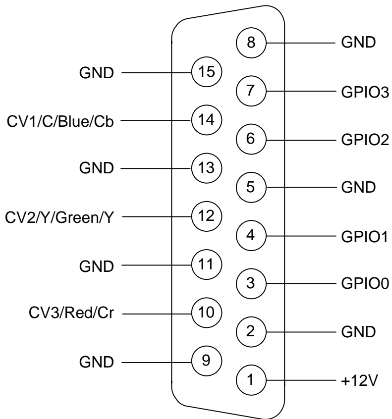
DSub 15-pin Female Samtec DSM-318-A-15
